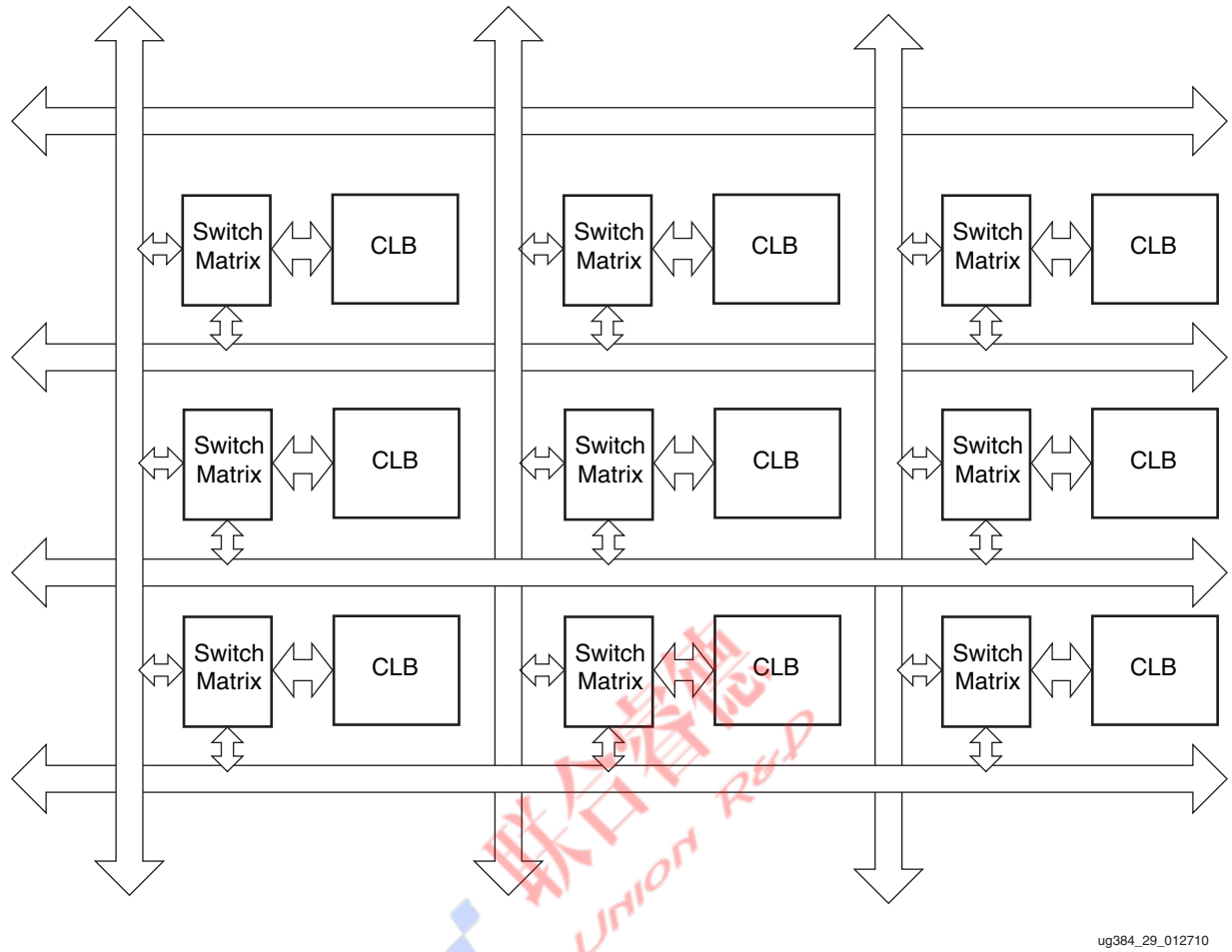
Figure 29: CLB Array and Interconnect Channels
